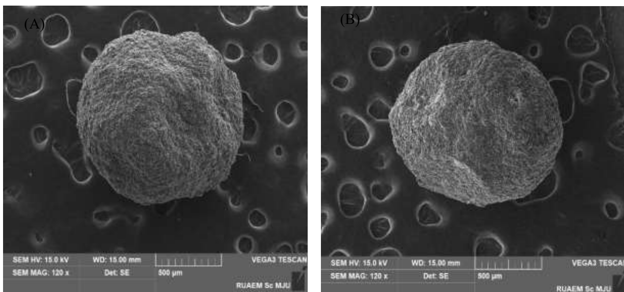
Figure 4. SEM micrographs (120× magnification) of PVA/Ag-BCH/SA composite beads before (A) and after (B) immersion in simulated sweat solution for 94 h.
