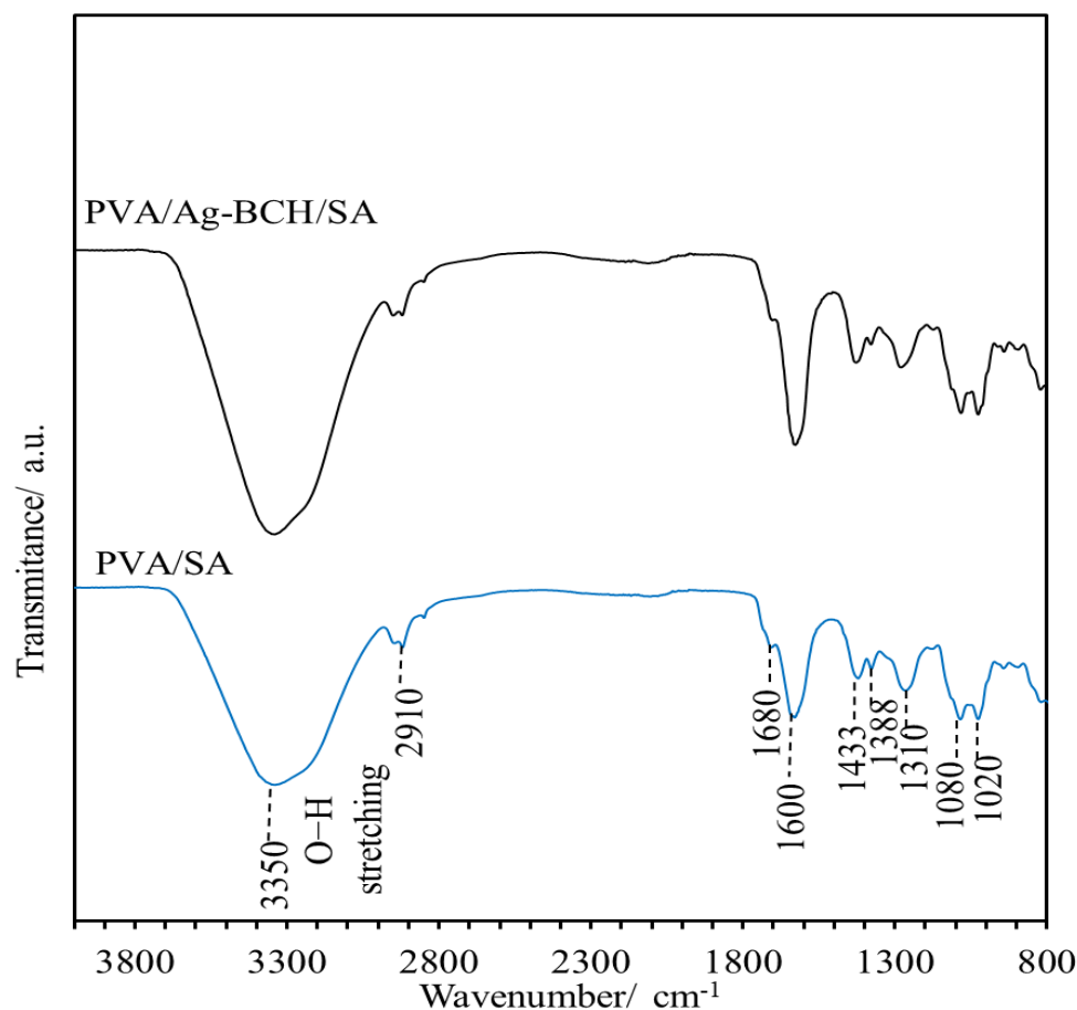
Figure 1. FTIR spectra of PVA/SA and PVA/Ag-BCH/SA composite bead.
