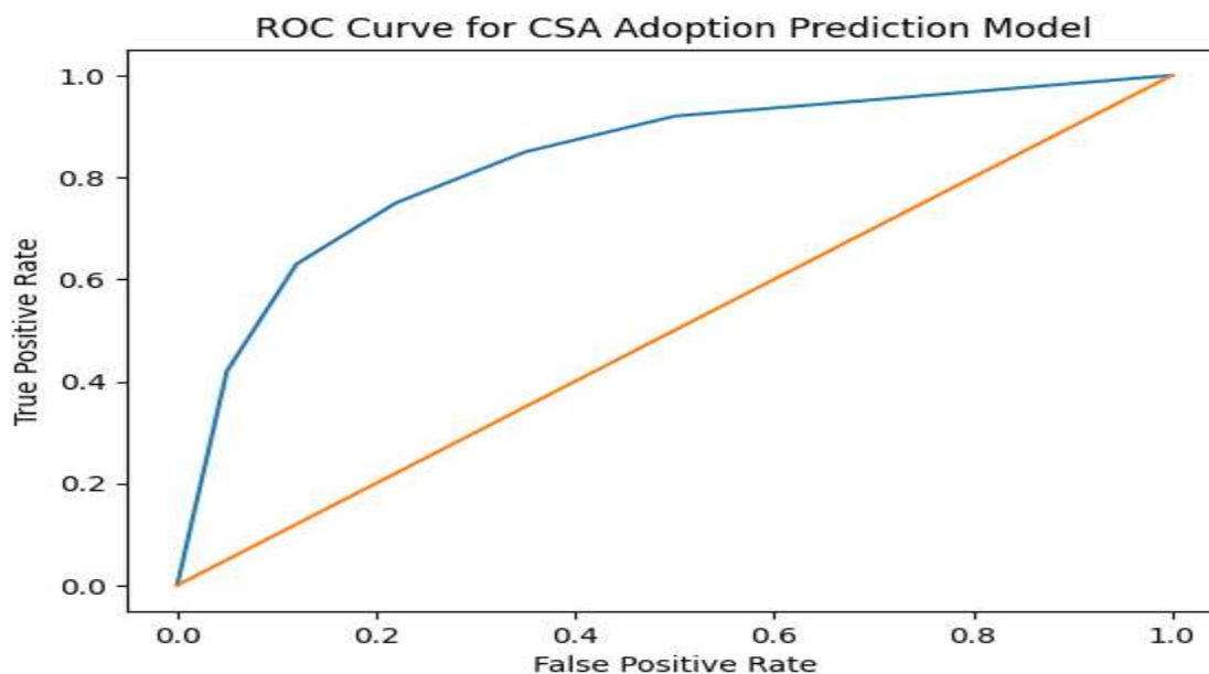
Figure 3: Receiver Operating Characteristic (ROC) curve for the CSA adoption prediction model
